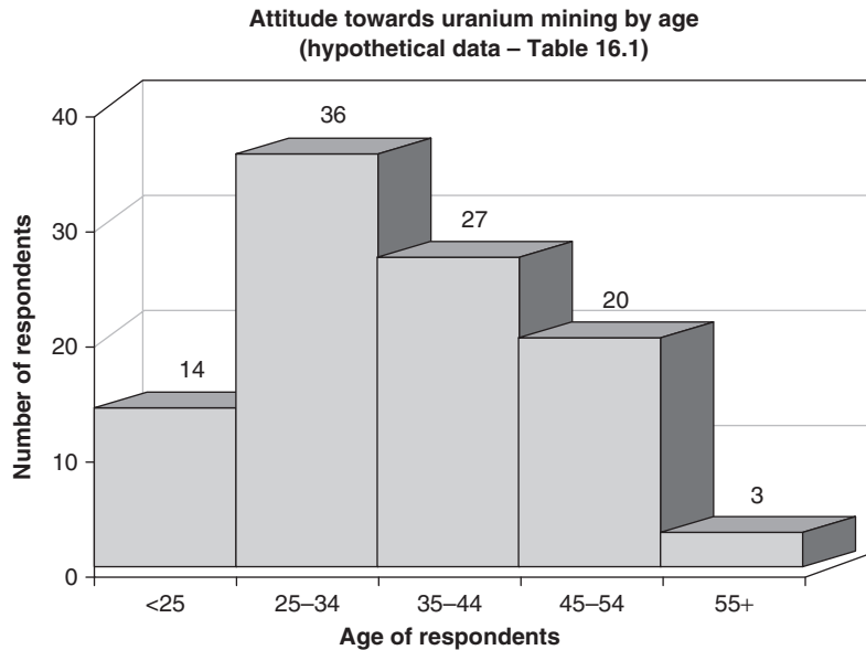
FIGURE 16.2b Three-dimensional histogram
