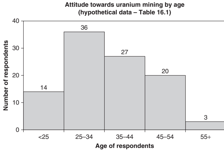
FIGURE 16.2a Two-dimensional histogram
