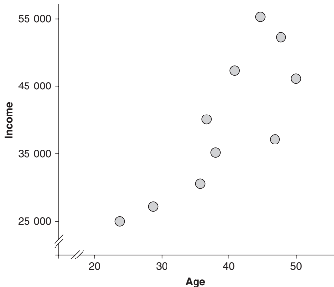
FIGURE 16.12 The scattergram
